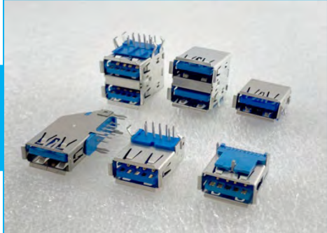
USB 3.0 CONN
